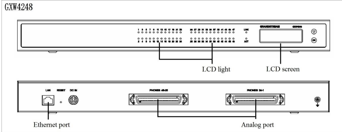
FIGURE 1: DIAGRAM OF GXW4216/24/32/48 PANEL
